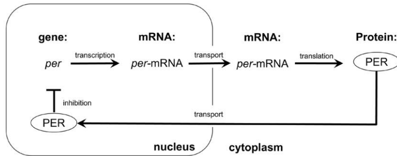
Figure 1. Proposed feedback mechanism for generating circadian oscillations.
