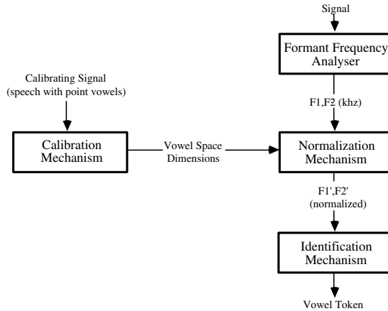
Fig. 2. The Gerstman vowel normalization model.
