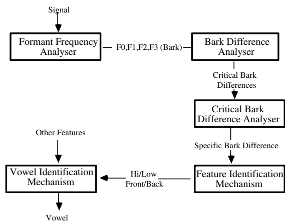
Fig. 3. The Syrdal/Gopal vowel normalization model.
