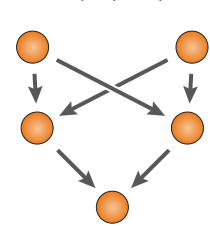
Multi-layer perceptrons
