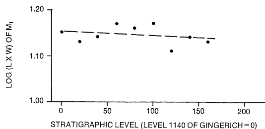
FIGURE 6. Plots of mean tooth size versus stratigraphic level for a segment of Gingerich's Hyopsodus lineage, as discussed and defined in the text. The regression indicates stasis during a period of supposed size decrease in the H. miticulus to H. lysitensis lineage. Dotted line is the least squares regression calculated from Gingerich's data.
