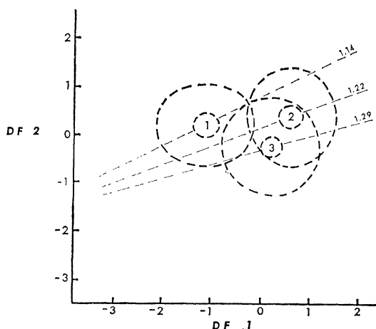
FIGURE 1. Three samples of Gypidula plotted on two canonical axes for two original variables. From Makurath and Anderson 1973. Numbers are centroids of the three samples in stratigraphic order; inner circles are 95% confidence intervals; outer circles represent one standard deviation around the mean canonical values. Dotted lines are contoured values of the simple shape ratio, y/x , plotted with respect to the axes. Although we see gradual change in the mean shape ratio, we find no gradualism for projections of centroids on either axis, or for general distances between centroids.
