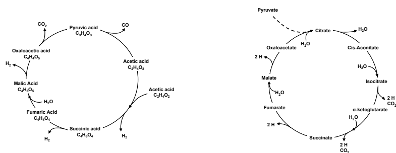
Figure 2. Two accounts of a key pathway of oxidative metabolism that recognized its cyclic organization. On the right is an early version of the Krebs cycle that was essentially correct, though incomplete. Its cyclic organization had been anticipated by Thunberg (1920), as shown on the left, but his conjecture that the crucial reaction produced succinic acid from acetic acid proved incorrect.
