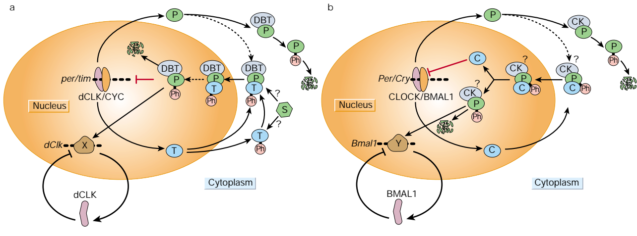
Figure 3 Drosophila and mammalian circadian clock. a , In Drosophila , a heterodimer of two bHLH–PAS domain-containing transcription factors, dCLK and CYC, binds to the E-box in per and tim promoters, promoting their transcription. DBT phosphorylates (Ph) cytoplasmic TIM-free PER protein (P) and triggers its degradation. As TIM (T) progressively accumulates, it binds to PER, prevents DBT activity, and stabilizes PER. Shaggy (S) phosphorylates TIM, and times the nuclear entry of the PER/TIM/DBT complex. TIM is later released from the nuclear PER/TIM/DBT complex, allowing repression of dCLK/CYC function. In the absence of TIM, DBT promotes the phosphorylation and degradation of nuclear PER, thereby derepressing dCLK/CYC function and starting a new wave of transcription from the E-box. dCLK constitutes another feedback loop by repressing its own transcription. PER promotes dClk transcription, although the transcription factor(s) that binds to the dClk promoter is currently unknown (X). b , In mammals, a heterodimer of two bHLH–PAS domain-containing transcription factors, CLOCK and BMAL1, binds to the E-box in Per and Cry promoters, and promotes their transcription. CK1ε phosphorylates cytoplasmic PER protein (P) and triggers its degradation. Three different mammalian PER proteins can bind to two mammalian CRY proteins and translocate into the nucleus; here CRY strongly represses CLOCK/BMAL1 activity, whereas PER promotes Bmal1 transcription. Bmal1 levels cycle, and the factor(s) that binds to its promoter is currently unknown (Y). Dotted lines represent delays; '?' denotes uncertainty in the step.
