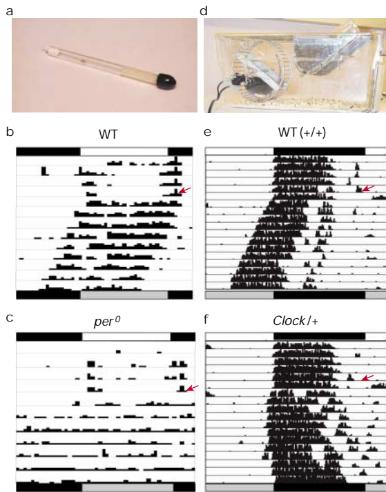
Figure 1 Assay of circadian activity rhythm in flies and mice. a , An infra-red beam and optical sensor automatically detect activity of a single fly placed inside a transparent tube and record it on an activity chart or actogram. Actogram of b , individual wild-type fly, and c , per 0 fly (bearing a loss of function mutation at per locus) recorded over several days. The flies were maintained under a 12-h light:12-h dark cycle for few days and then transferred to complete darkness at the time indicated by a red arrow. The per 0 mutation stops the clock and results in arrhythmic activity under constant condition. d , Wheel-running activity of individually caged mice gives a measurement of circadian activity rhythm. e , Wild-type (+/+) and f , mutant mice (+/−) containing one copy of the mutated Clock gene both show similar activity pattern under an entraining light:dark condition. After transfer to constant darkness, the wild-type mouse exhibits a rhythm slightly shorter than 24 h, whereas the mutant mouse has a longer period of activity rhythm. Robustness of the assay enabled detection of this mutant in the original screen. Homozygous Clock/Clock mice behave in a way that is similar to per 0 flies under extended darkness.
