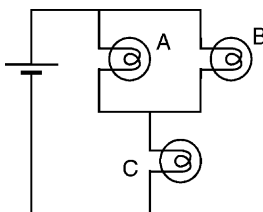
Fig. 2. A network of light bulbs.
