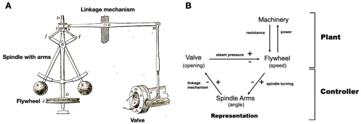
Figure 22. A. Watt's design of the Watt governor. Redrawn from Farley (1827). B. Schematic representation showing how spindle arms represent the speed of the machinery and how this representation is used to affect the valve opening.
