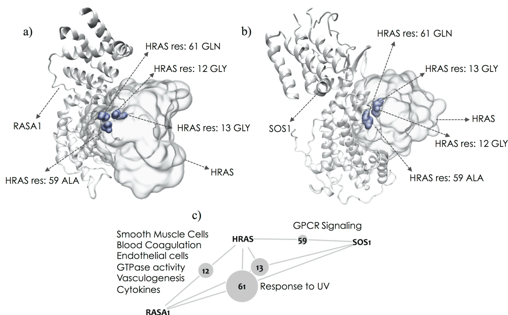
Figure 3. The RASA1–HRAS complex (a) and the SOS1–HRAS complex (b) show that both interactors utilize the same binding site on HRAS. Residues 12, 13, 59 and 61 on HRAS that participate in the interface region of these interactions are highlighted in blue. Residue 12 mediates the HRAS-RASA1, residue 59 mediates the HRAS-SOS1 interaction, and 13 and 61 participate in both interactions. The small network (c) provides a schematic of the residues mediating particular interactions. The grey nodes represent the residues. Their sizes are proportional to the frequency with which they are mutated in the TCGA cohort. Functions predicted to be specifically altered by mutations at each interface are listed on the edges.
